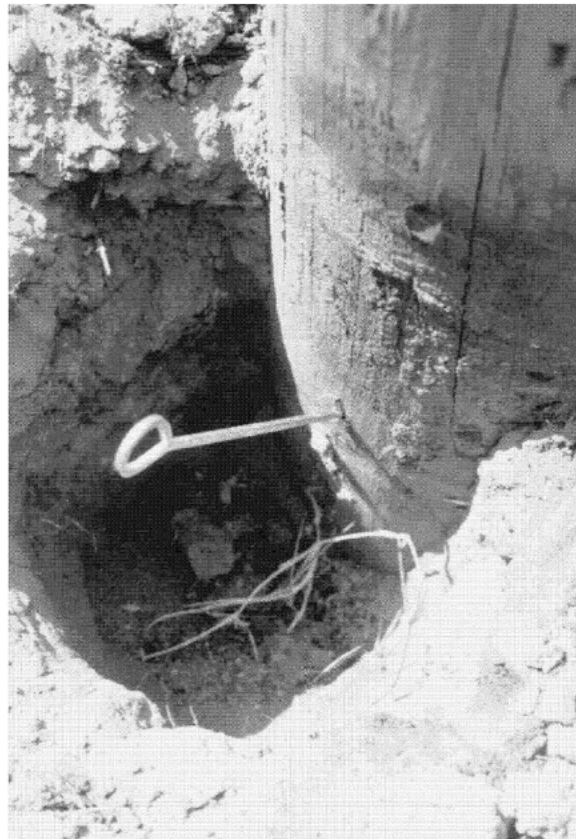
Figure 3. Using a Shell Thickness Gauge
