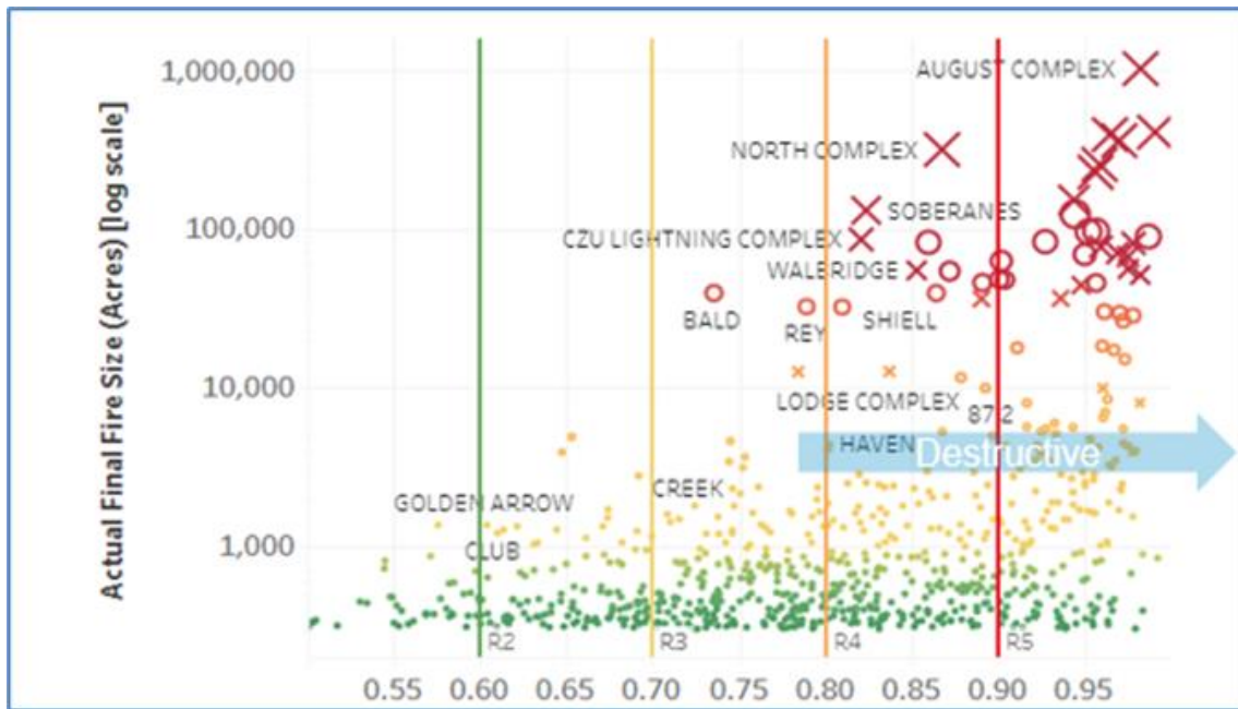
FIGURE PG&E-6.2.2-6: TECHNOSYLVA SIMULATION FPI R SCORE AND DESTRUCTIVE FIRE RELATIONSHIP
