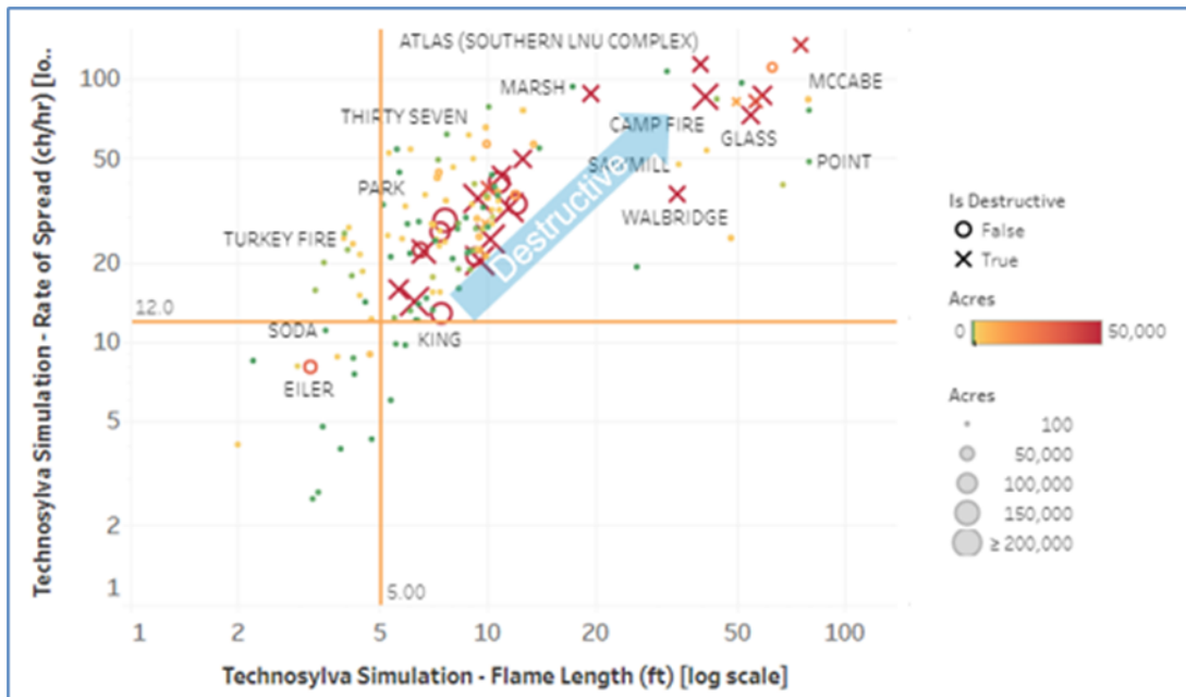
FIGURE PG&E-6.2.2-7: FPI R SCORE TECHNOSYLVA SIMULATION AND DESTRUCTIVE FIRE RELATIONSHIP
