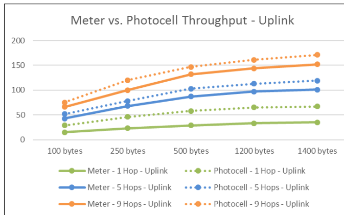
Figure 3. Average Network Throughput (kbps) Comparison – Uplink
