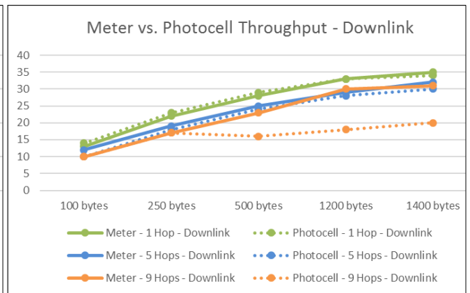
Figure 2. Average Network Throughput (kbps) Comparison – Downlink
