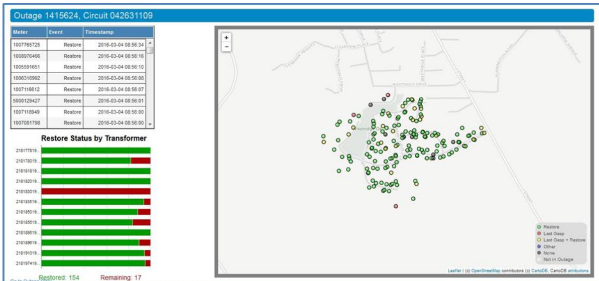
Figure 17. Nested Outage
