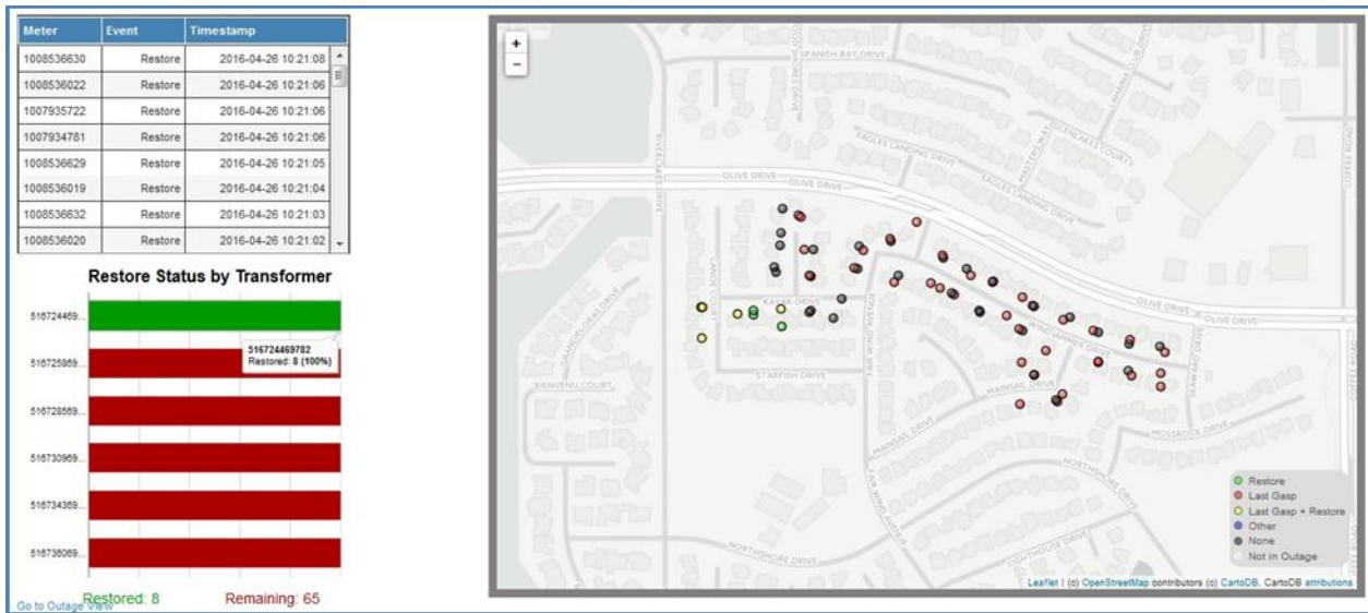
Figure 16. Restoration Dashboard
