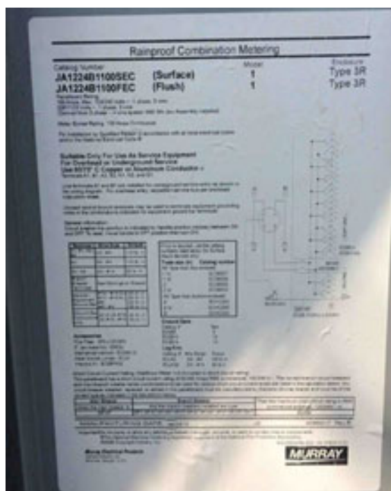
Figure 16 Electric Meter Panel Label – Picture Set 3 (2)
