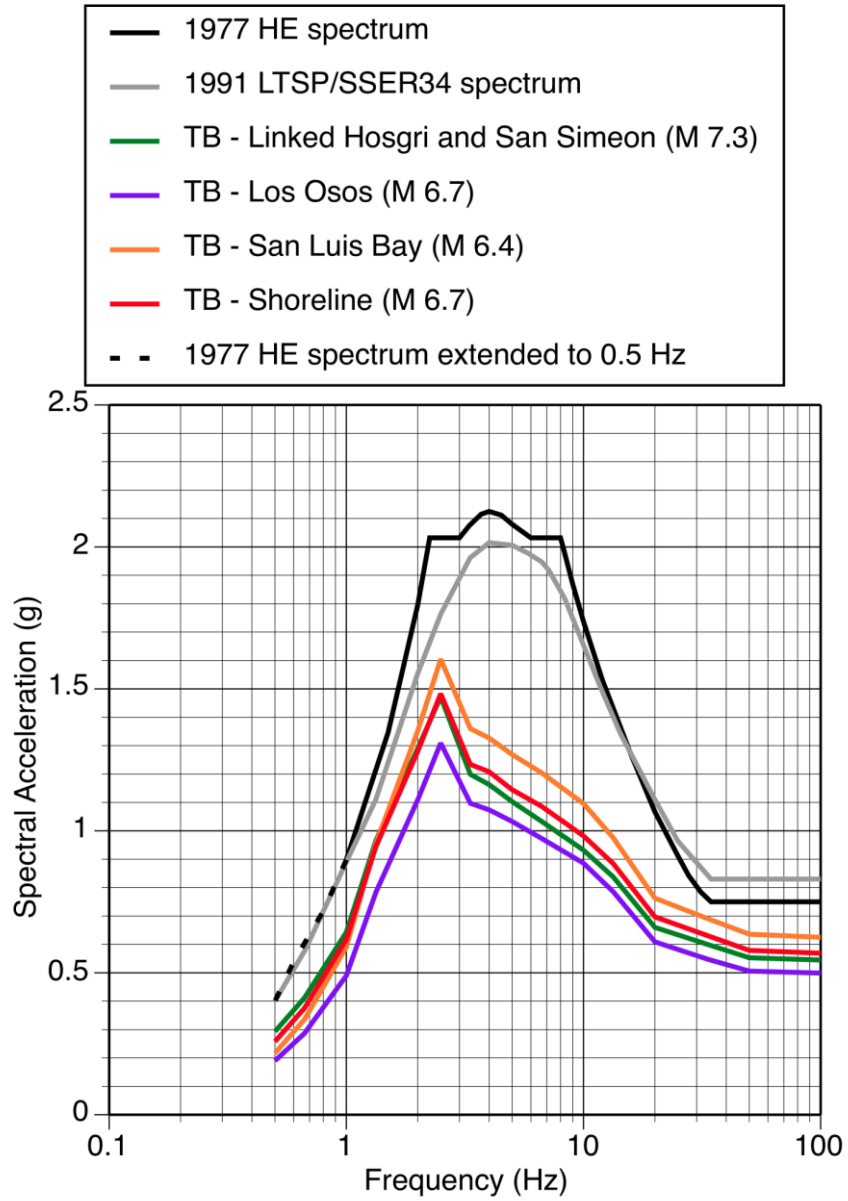
The 84th Percentile Deterministic Ground Motions for Four Fault Scenarios Compared to the 1977 Hosgri Earthquake (HE) and the 1991 LTSP/SSER 34 Spectra for the DCP Turbine Building
